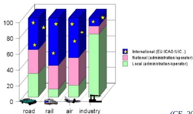
Estimated shares in noise reduction
